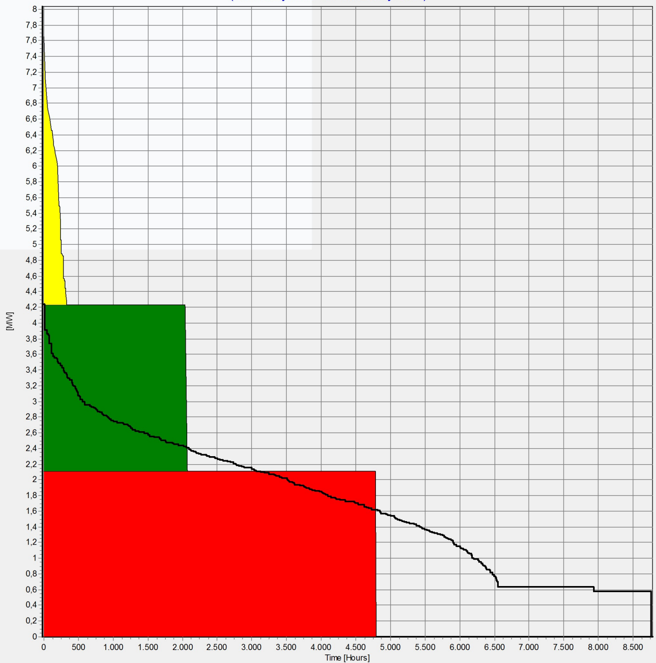
Duration curve for heat demand (1. January 2011 to 1. January 2012)
