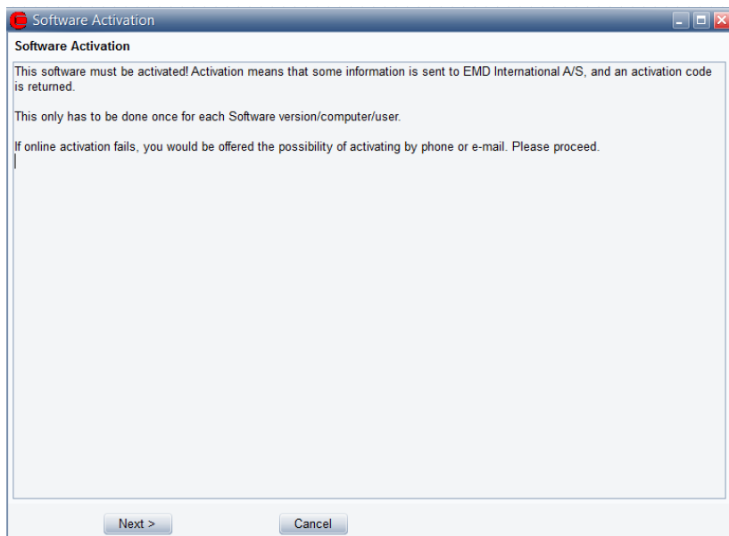
Figure 1.5: Software Activation
