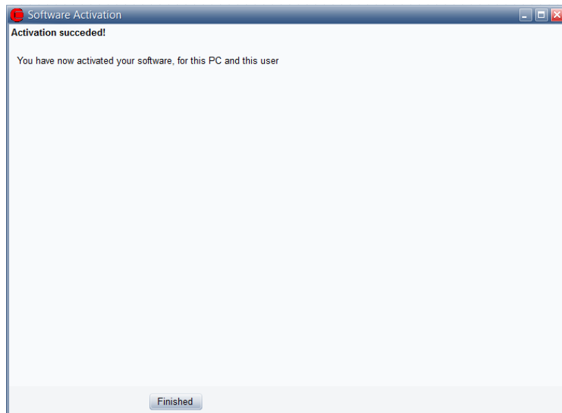
Figure 1.11: Activation succeeded
