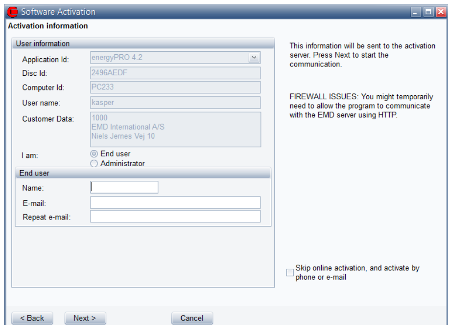
Figure 1.6: Activation information
