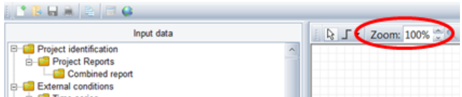
Figure 1.21: Setting zoom-factor
