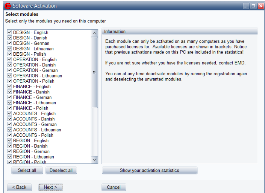
Figure 1.9: Select modules
