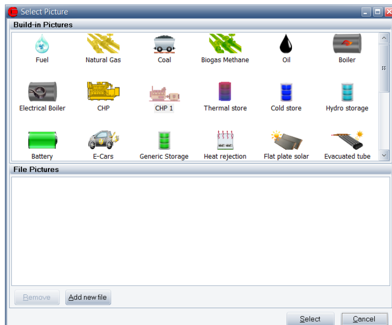
Figure 1.30: Select Picture
