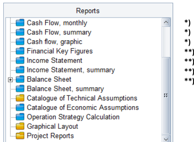
Figure 2.151: Reports financial
