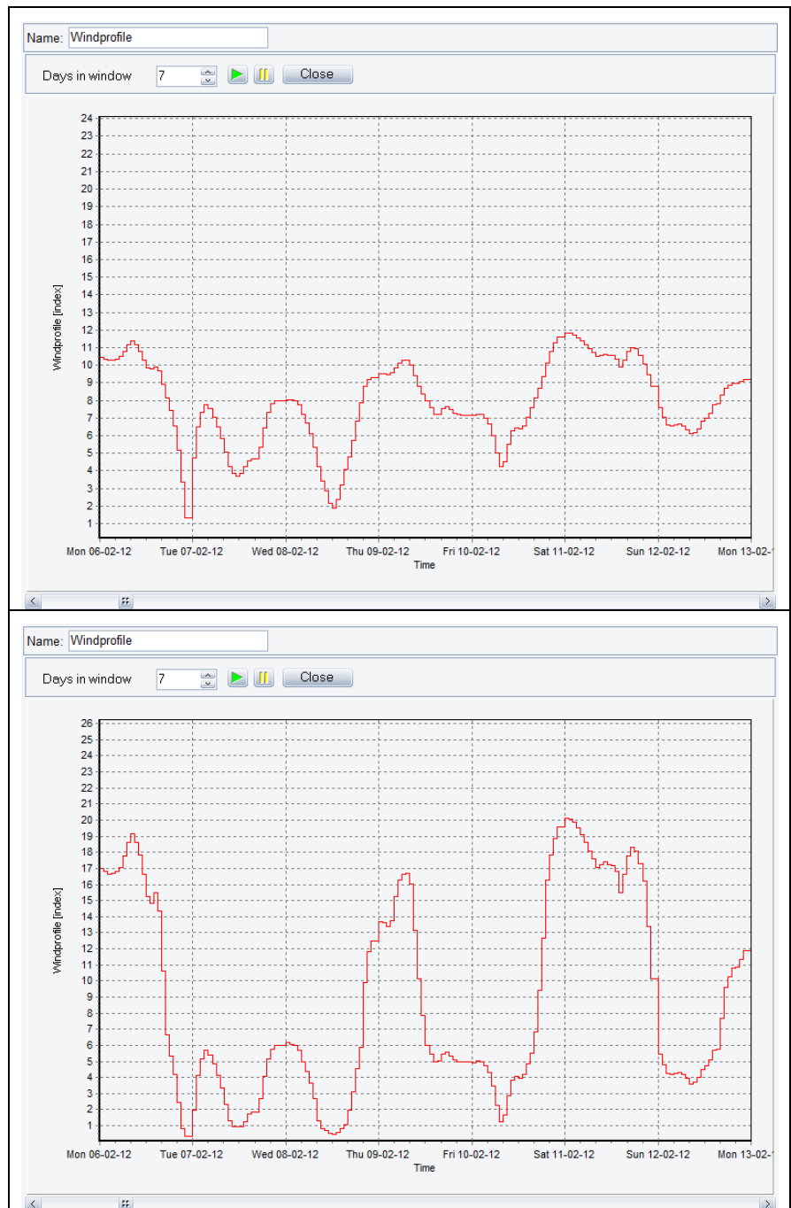
Figure 2.26: Time series function example shown graphically. Upper before modifying in conversion table. Lower after modifying in conversion table.
