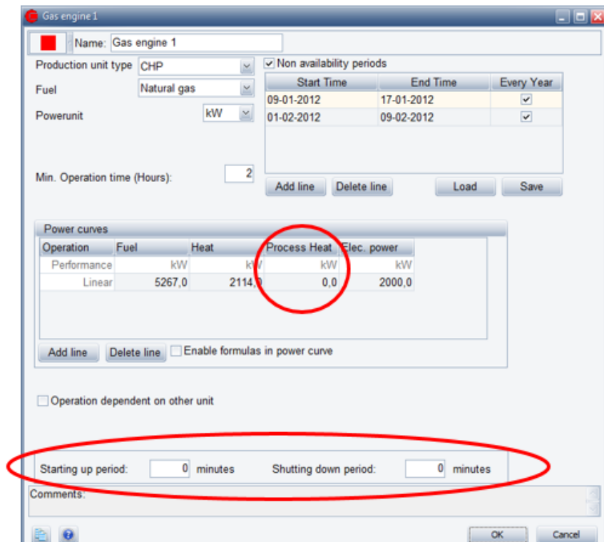
Figure 2.9: Production unit with two advanced options enabled. Starting up and shutting down periods shown and process heat available.
