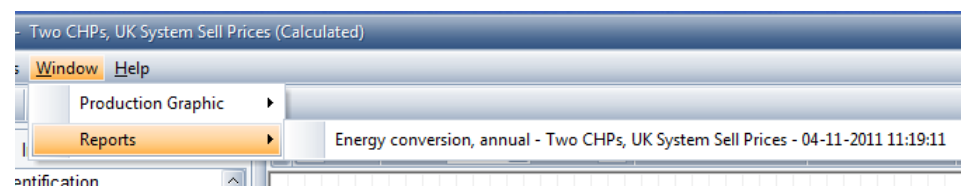
Figure 2.6: User Interface
