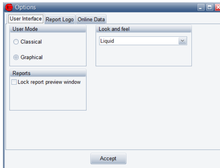
Figure 2.3: User Interface
