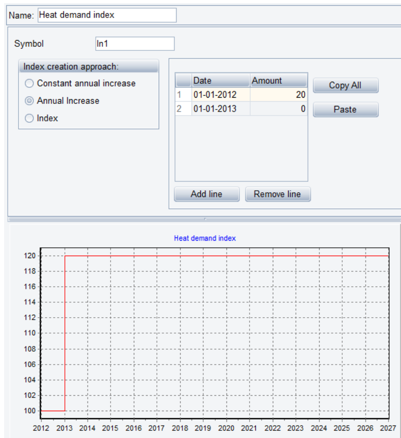
Figure 2.27: Index – example
