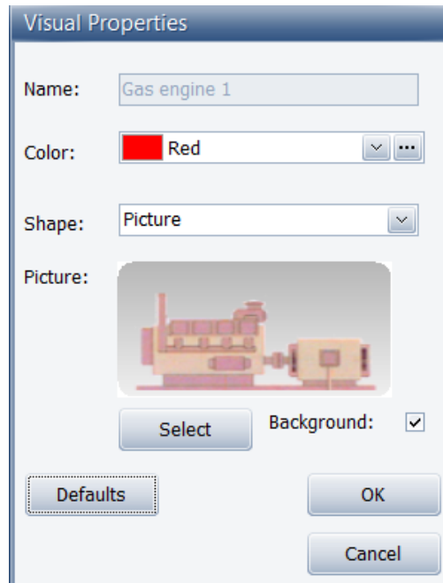
Figure 1.29: Visual Properties
