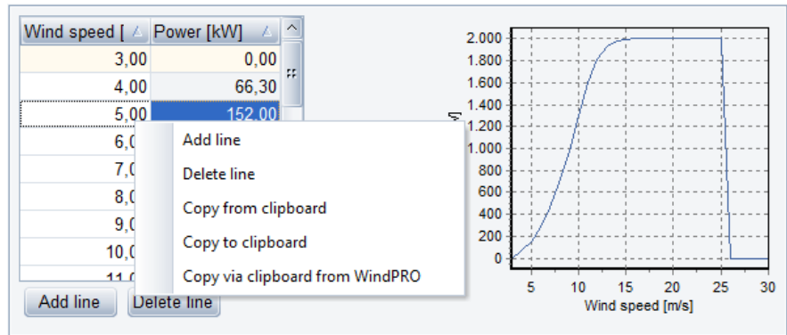
Figure 2.73: The power curve. Values can be copied from clipboard, including park power curve calculated in WindPRO
