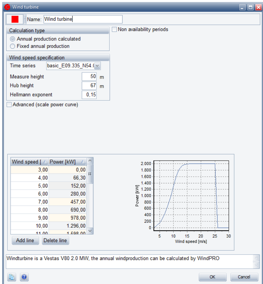
Figure 2.74: Wind farm, “Annual production calculated”, not advanced
