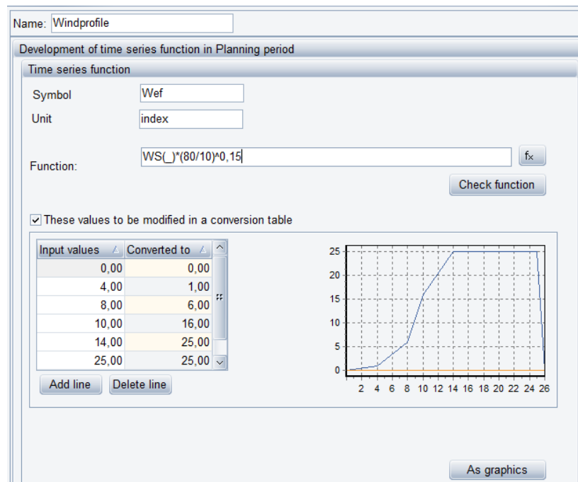
Figure 2.25: Time series function example, where a wind velocity in 10 meters height is modified to wind velocity in 80 meters height and finally converted to energy output using a conversion table, which describes the power curve of a wind turbine.
