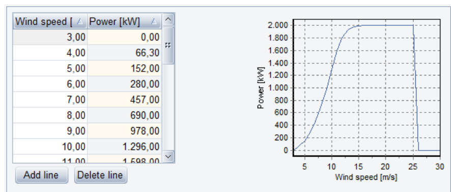
Figure 2.72: The power curve of the wind farm
