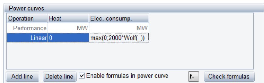
Figure 2.51: Power curve, formula enabled example
