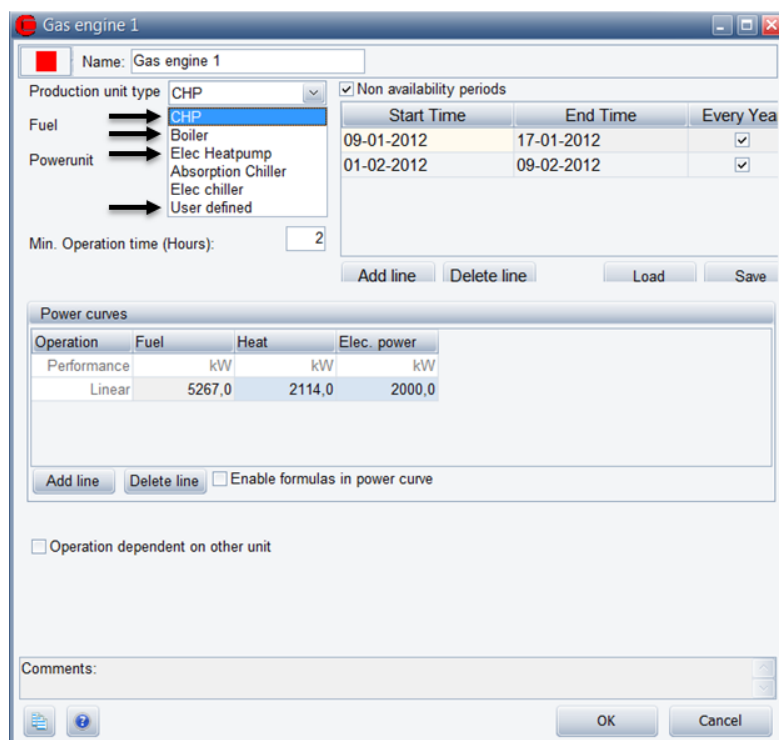
Figure 2.95: Net Heat production costs are only calculated for Heat producing Production units.
